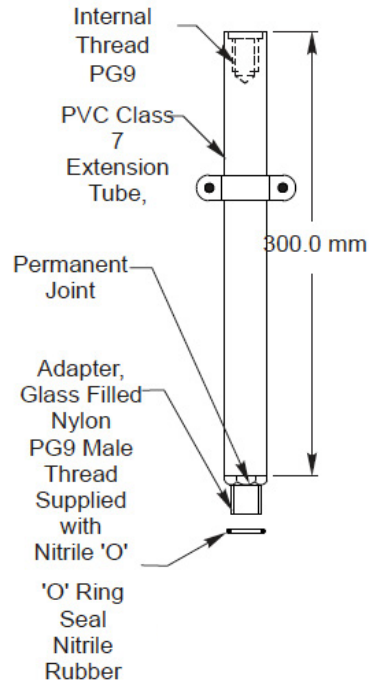
Extension Assembly
