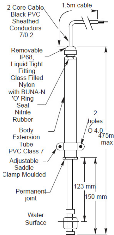
Switch Assembly
