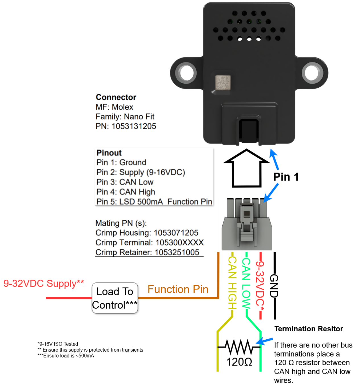
FIGURE 3 WIRING EXAMPLE
