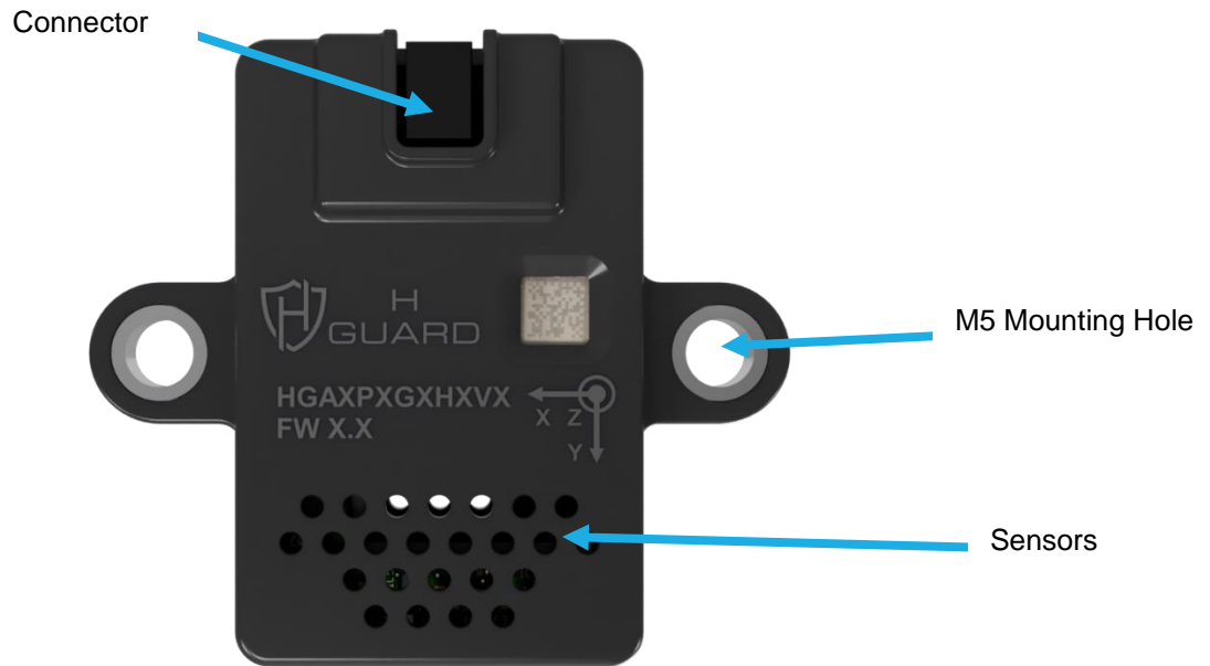
FIGURE 5 EXTERNAL FEATURES
