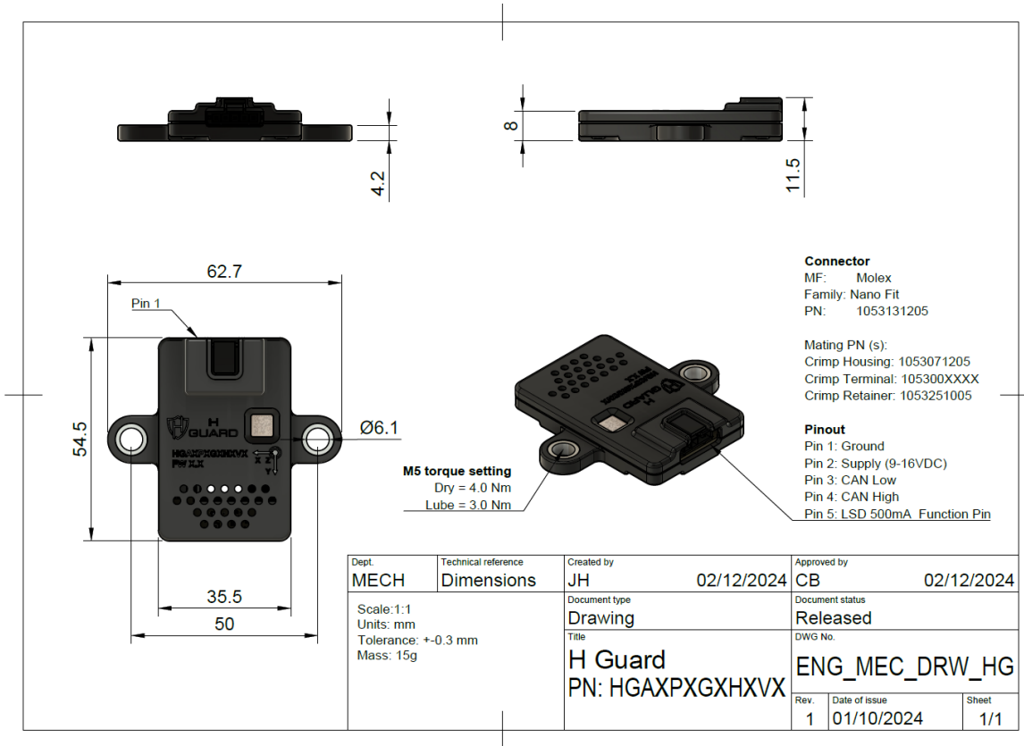
FIGURE 4 SENSOR DIMENSIONS
